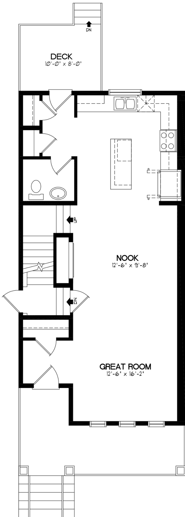
MAIN FLOOR - 773 SQFT
