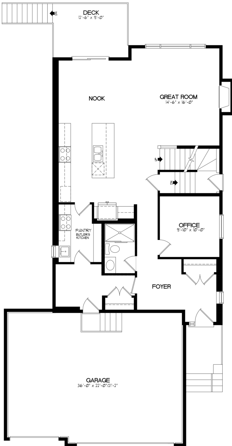
MAIN FLOOR - 1220 SQFT
