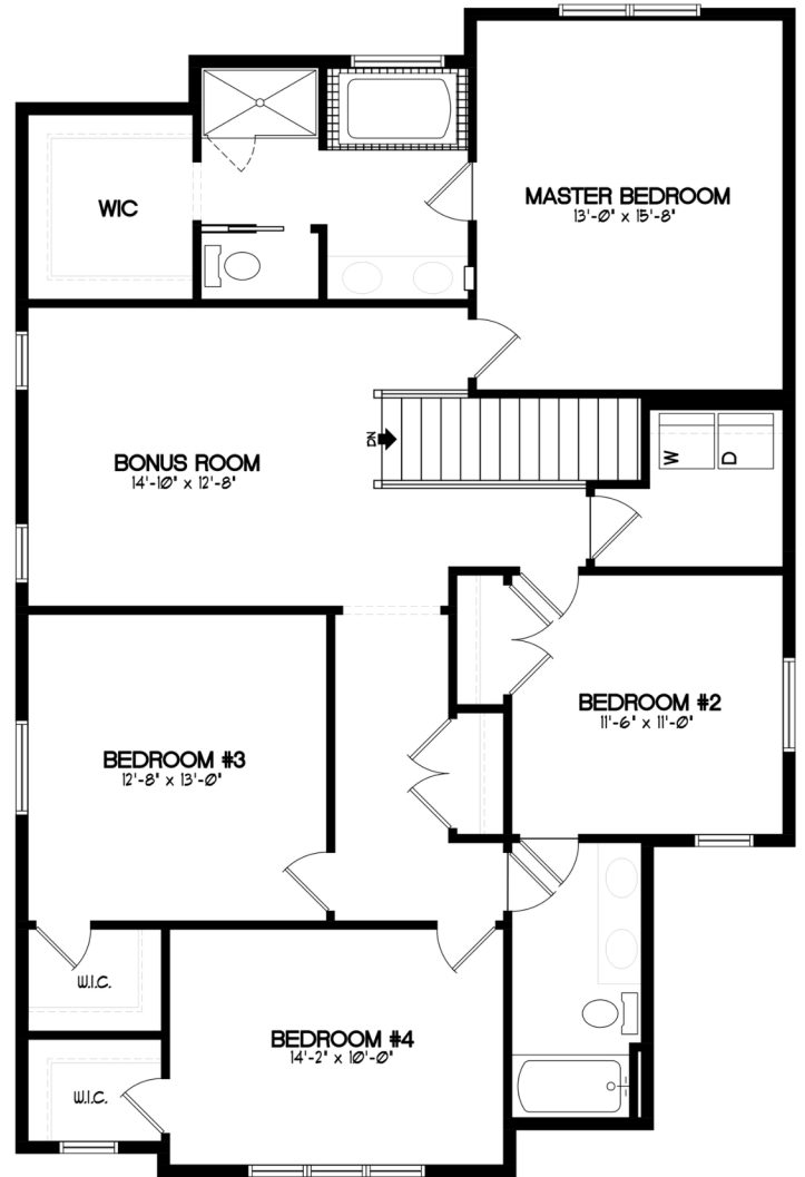
UPPER FLOOR - 1440 SQFT
