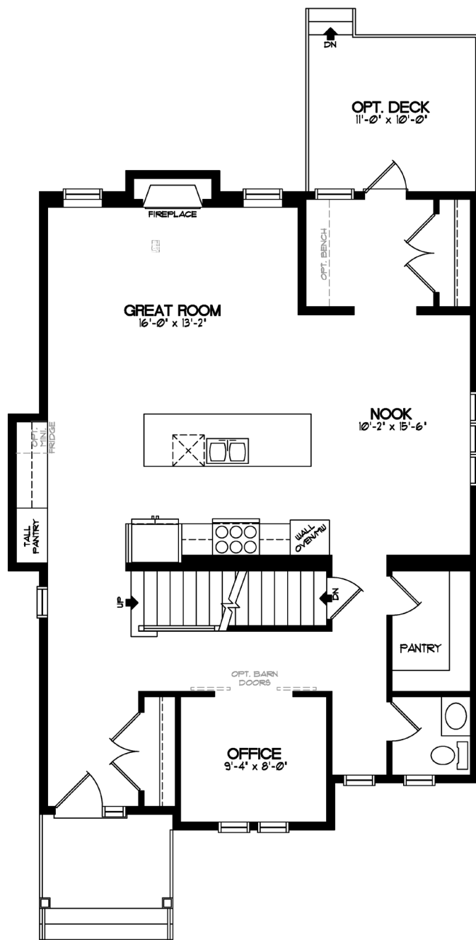
MAIN FLOOR - 1123 SQ. FT.
