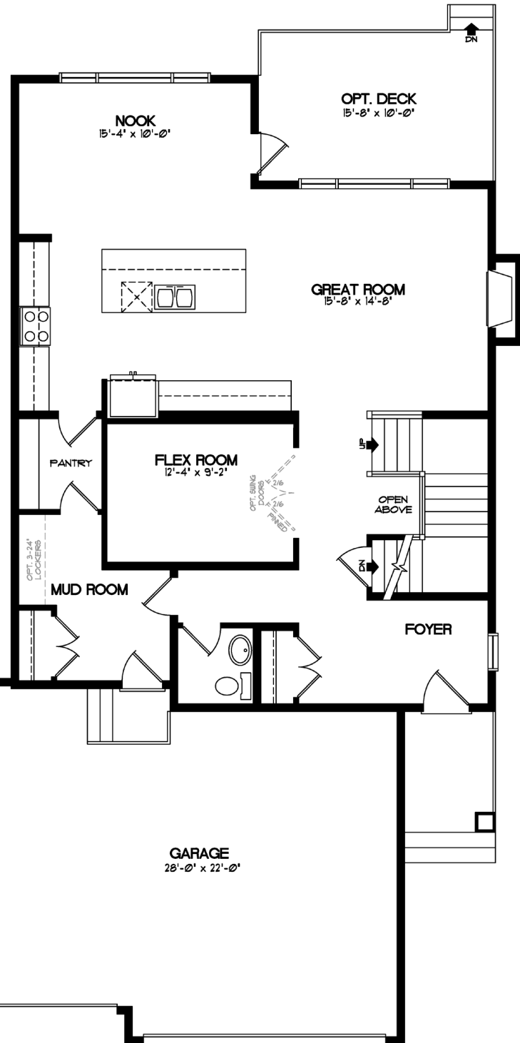
MAIN FLOOR - 1219 SQ. FT.
