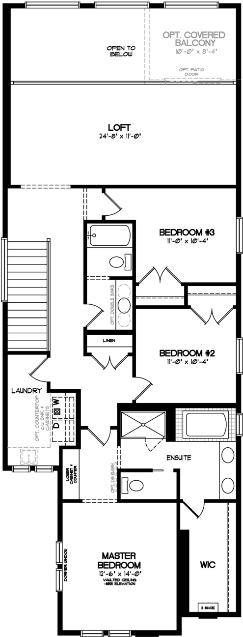
UPPER FLOOR - 1425 SQ. FT.
