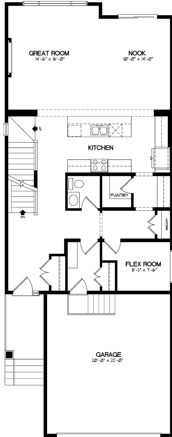
MAIN FLOOR - 1124 SQ. FT.
