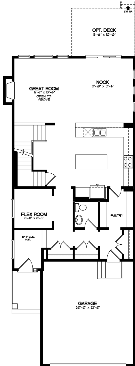
MAIN FLOOR - 1131 SQ. FT.
