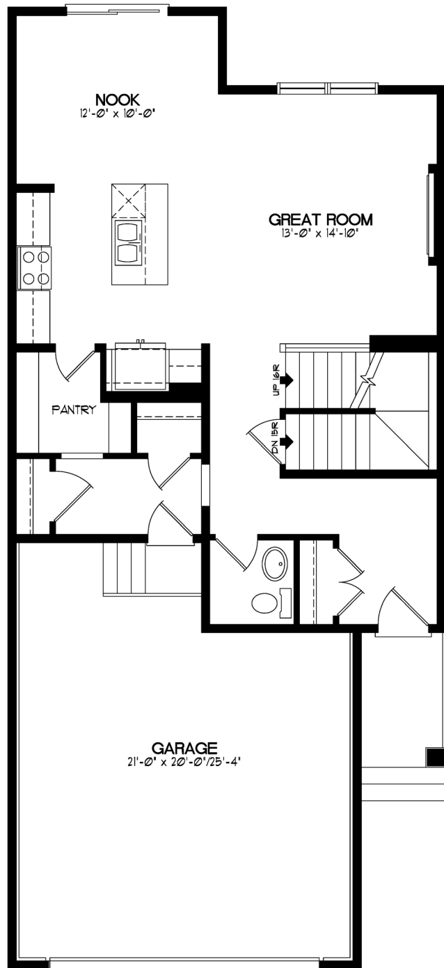
MAIN FLOOR - 844 SQ. FT.
