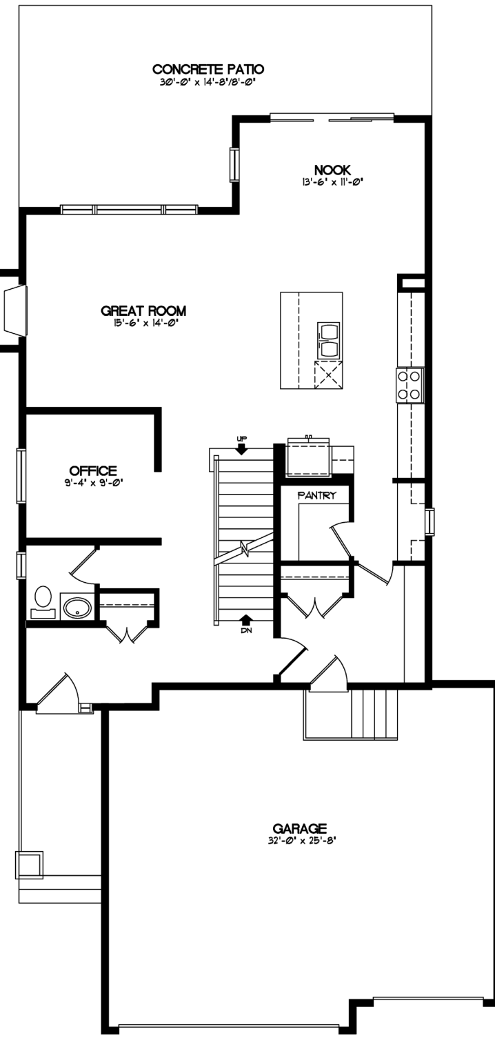
MAIN FLOOR - 1162 SQ. FT.
